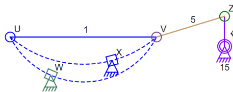
Figure 30. Invalid Sliding Connector Curved Path
