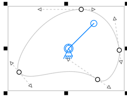
Figure 25. Cam Tutorial Spline Shaped and Positioned
