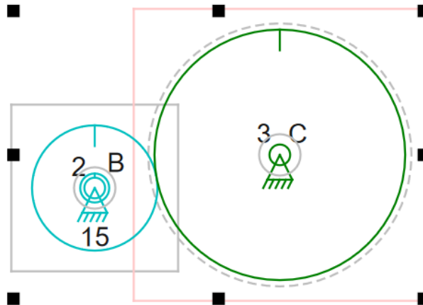
Figure 36. Gear Tutorial with a 1:2 Ratio
